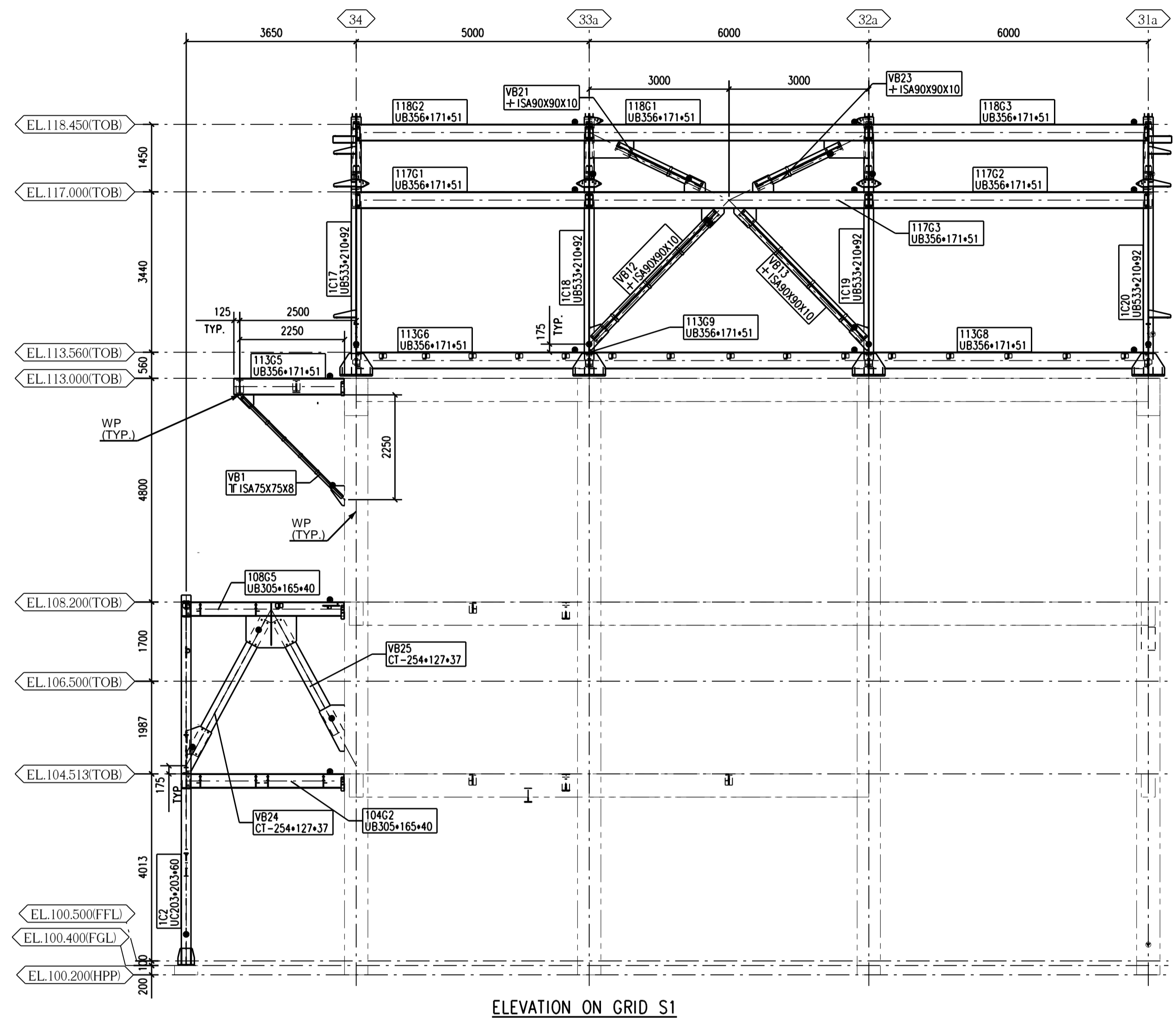
ELEVATION ON GRID S1
