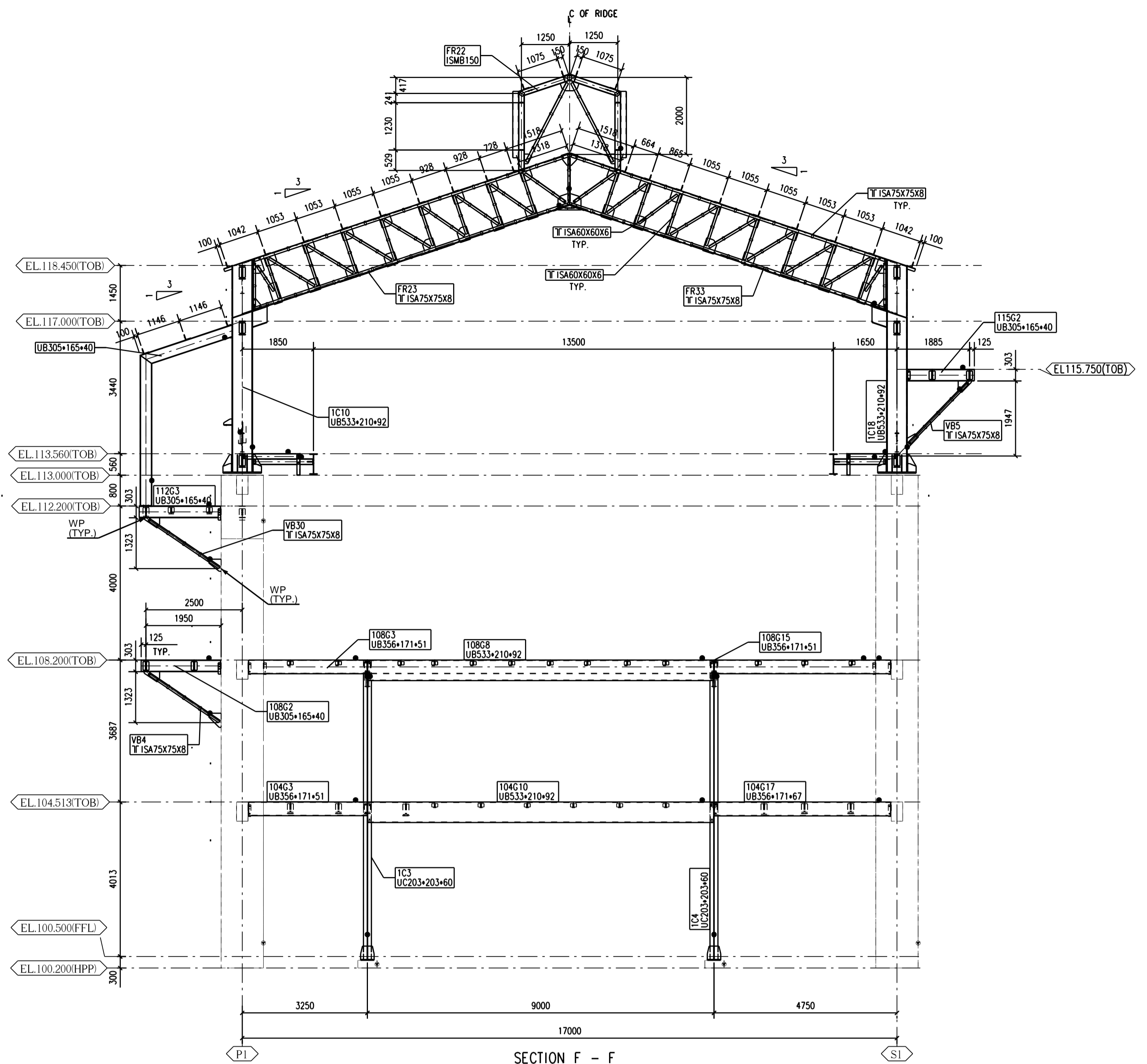
SECTION F - F
