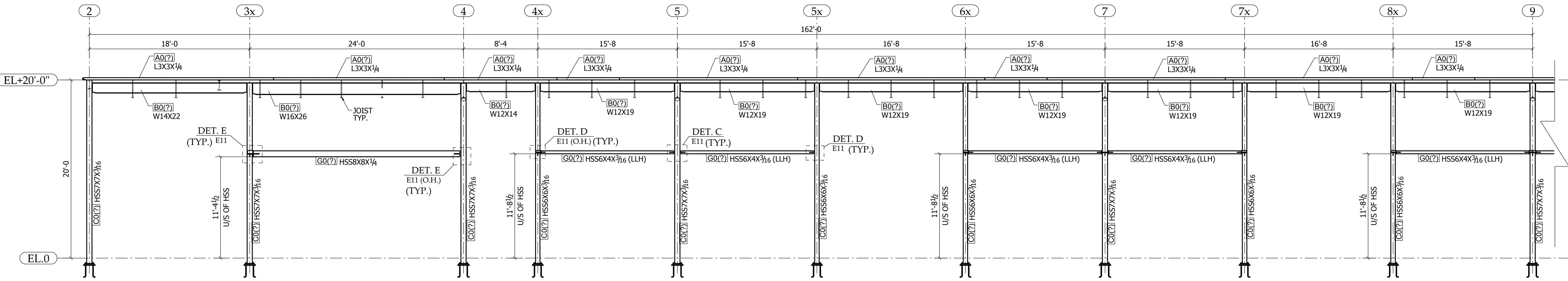
ELEVATION ALONG GRID LINE A
